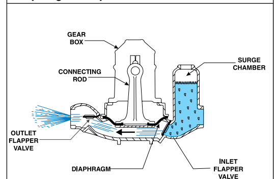
Diaphragm Pump — Discharge Stroke
