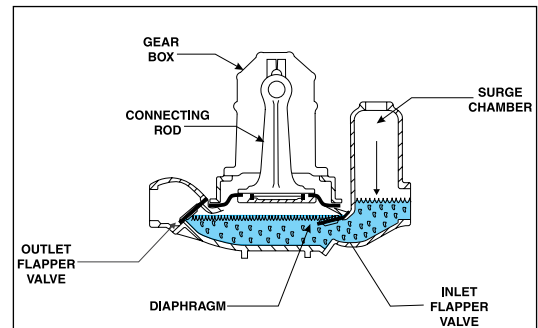
Diaphragm Pump — Suction Stroke
